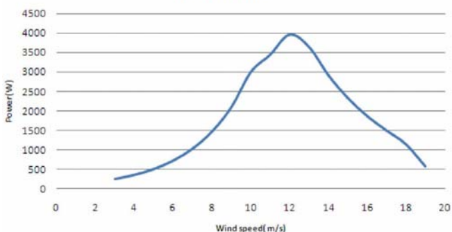
Power curve
